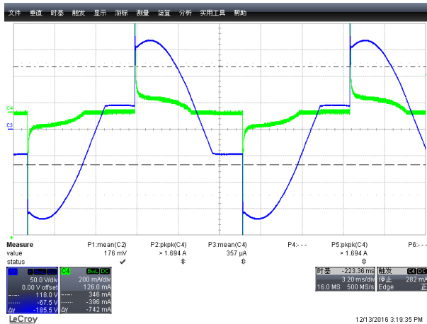
Input AC Current vs Dimmer Phase ( V_{in}=120V_{AC}/60Hz , Conduction Angle 110deg)
