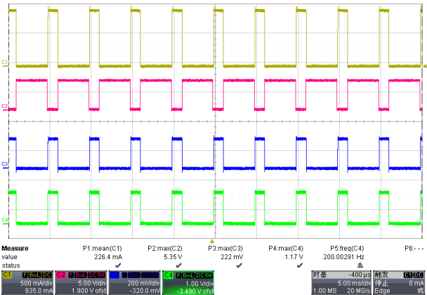
Frequency=200Hz, duty=70%
