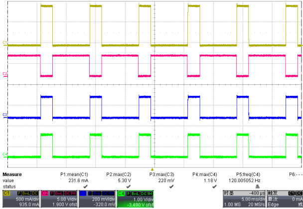
Frequency=120Hz, duty=70%
