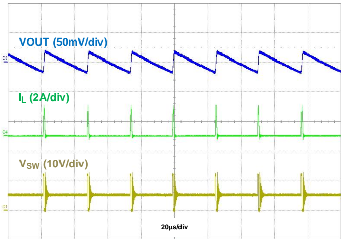
Figure 10. Output Voltage Ripple, IOU = 50mA VIN = 12V, VOUT = 5V USM f SW = 800kHz
