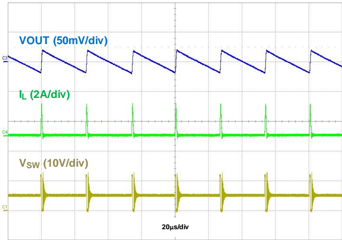
Figure 8. Output Voltage Ripple, IOU = 50mA VIN = 12V, VOUT = 5V PFM f SW = 800kHz
