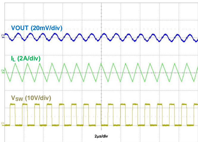
Figure 12. Output Voltage Ripple, IOU = 50mA VIN = 12V, VOUT = 5V PWM f SW = 800kHz
